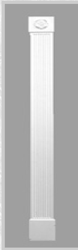
P1 2070 X 180 X 43 PILASTER
